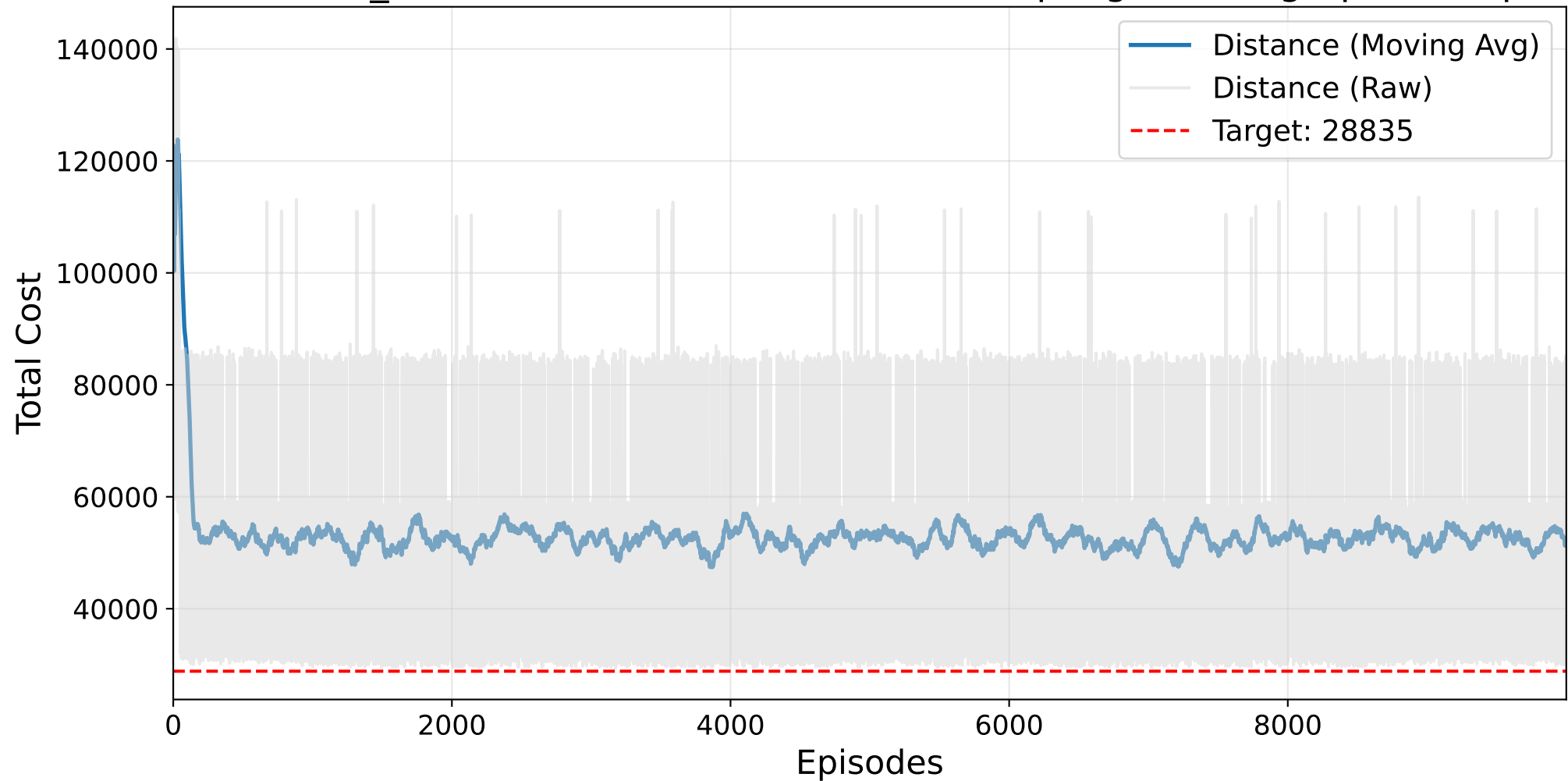
Final NO_MASK Masked AutoRL-SOP (Resampling) Training - p43.3.sop
